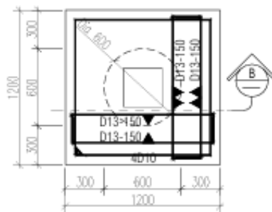
Figure 1. Pile Cap Arrangement
