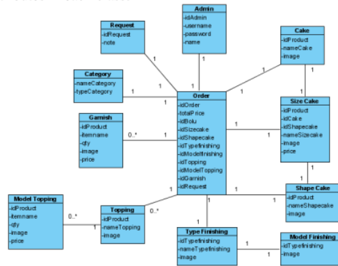
Figure 7. Class Diagram
