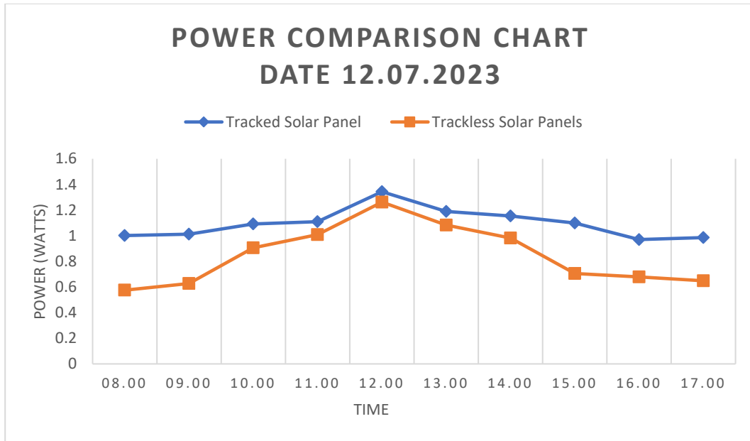
(c) Figure 13. Solar Panel Power Measurement Chart (a) Solar Panel Power Measurement Chart (b) Solar Panel Power Measurement Chart (c)
