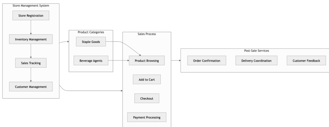
Figure 1. UML Diagram
