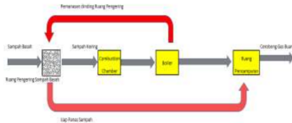
Figure 2 Scheme of Dryer System Method B
