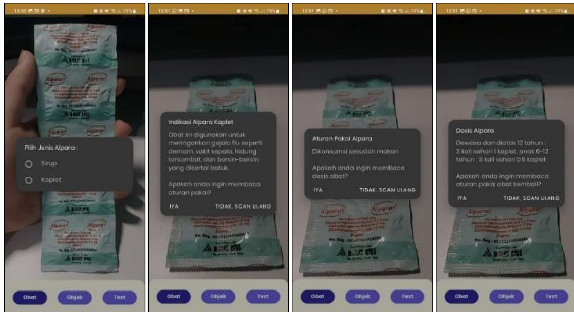
Figure 3. Drug Detection
