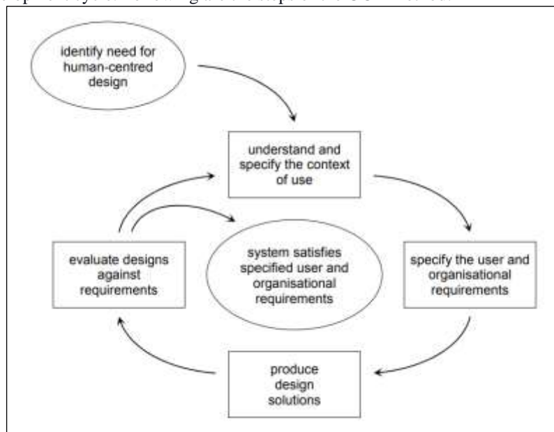
Figure 1. UCD Method [16]
