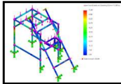
Figure 9. Results of Von Misses Stress Analysis
