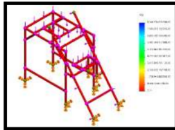
Figure 11. Results of Factor of Safety Analysis
