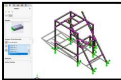
Figure 4. Selection of Fixed Geometry in Frame Testing
