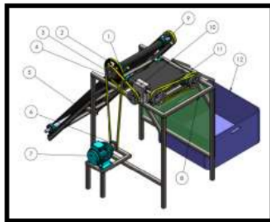
Figure 2. River Flow Garbage Transport Machine
