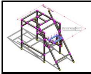
Figure 7. Giving Force Load on the Underframe
