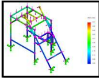
Figure 10. Displacement Analysis Results
