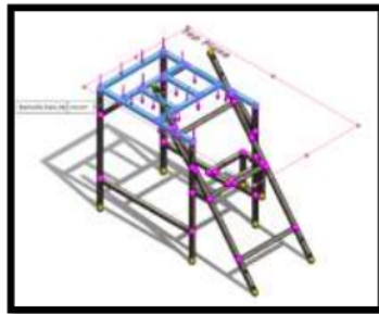
Figure 5. Giving Force Load on the Upper Frame
