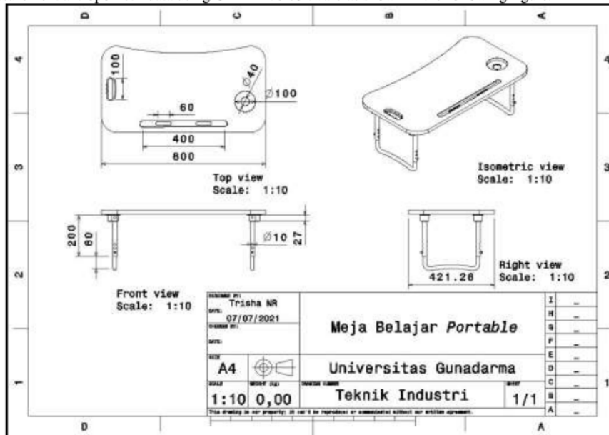
Figure 1. Desain Portable Desk Study
