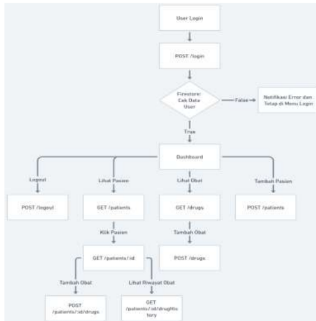
Figure 1. Admin Health Post Wireframe
