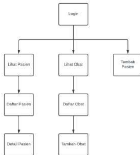
Figure 2. Navigation Structure
