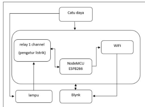
Gambar 3.1 Diagram blok
