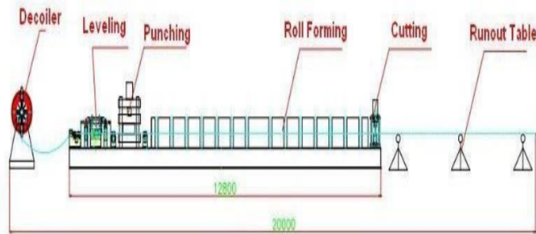
Gambar 8. Roll Forming
