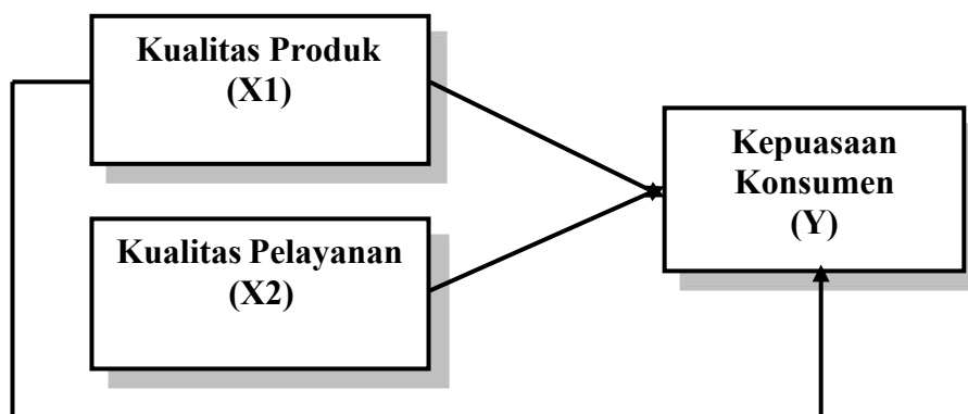
Gambar 1. Paradigma Penelitian
