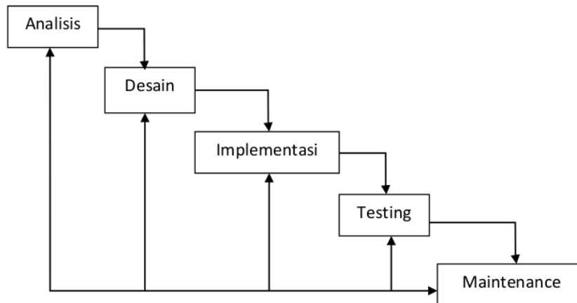
Gambar 1. Siklus Sistem Informasi, Diagram Waterfall .
