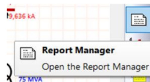
Gambar 12. Report Manager
